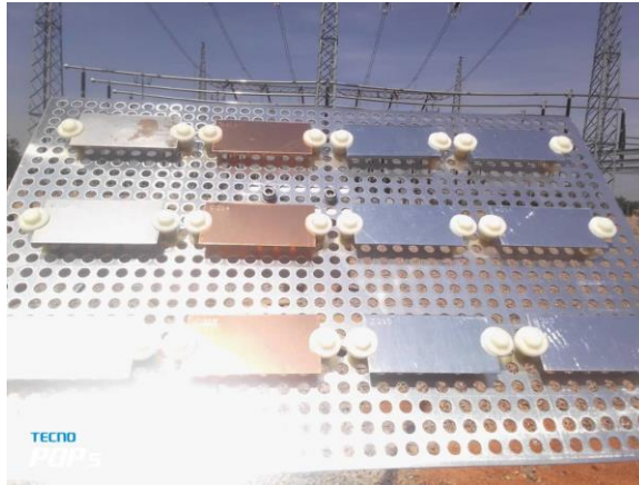
Figure 34: Echantillonneur de corrosion / Corrosion sampler.
