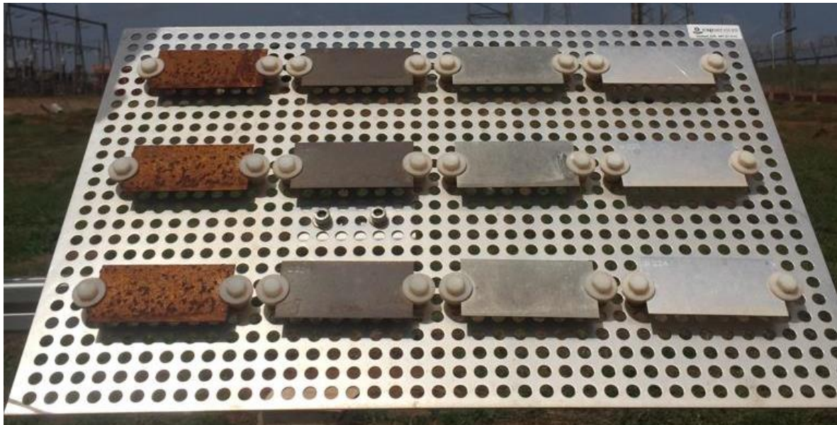
Figure 92: Echantillonneur de corrosion / Corrosion sampler.
