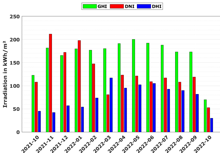
Figure 21: Totals mensuels de l'irradiation / Monthly irradiation sums.
