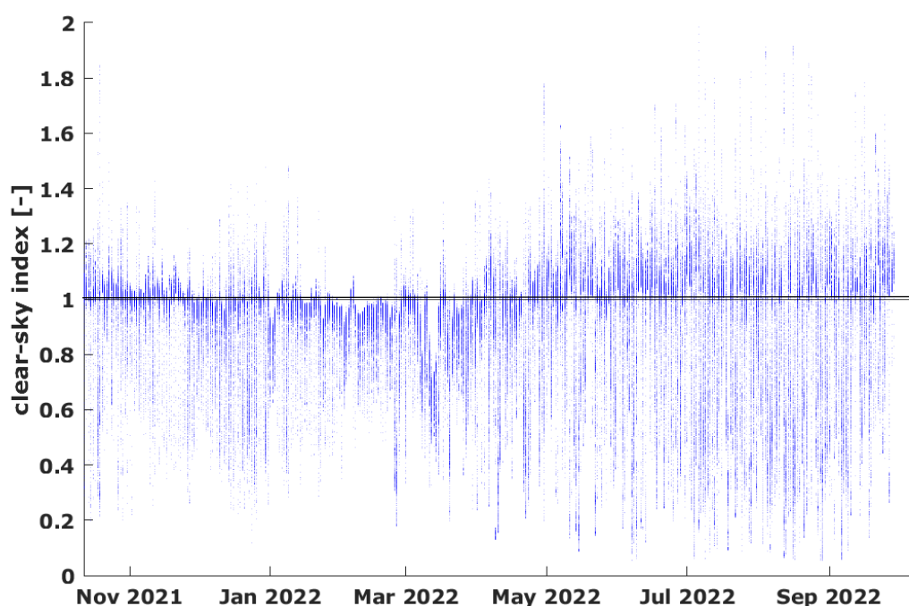
Figure 39: Indice ciel clair pour la GHI (resolution 1min) / Clear-sky index for the GHI (1min resolution).
