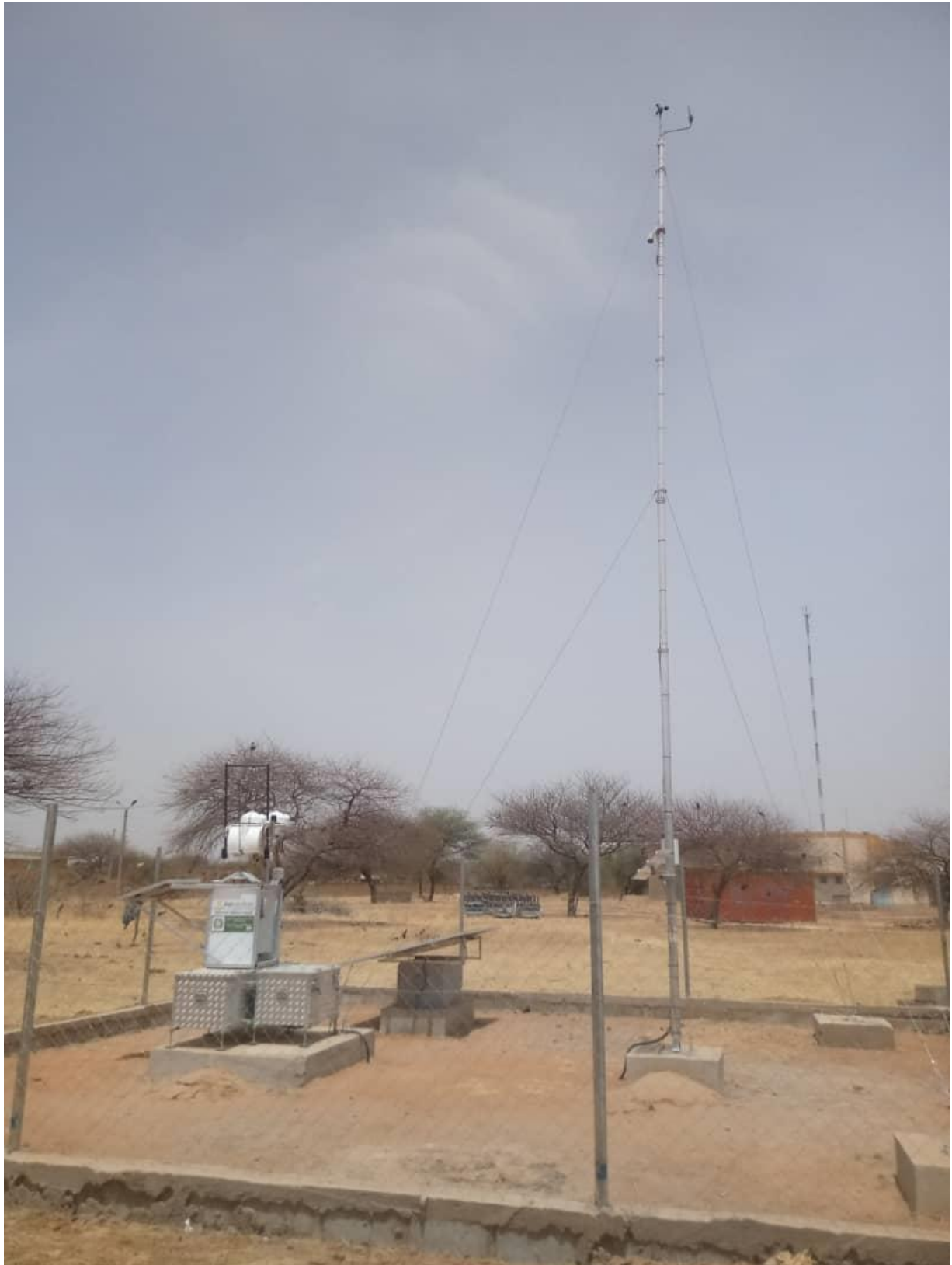
Figure 92 : Vue générale de la station / General view of the station.
