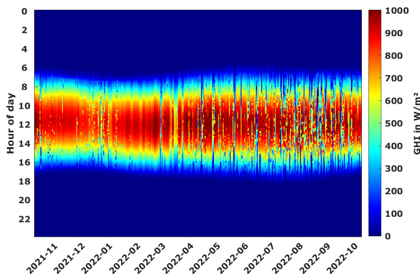
Figure 23: Intensité de la GHI / GHI irradiance intensity.
