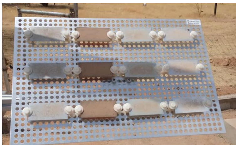
Figure 88: Echantillonneur de corrosion / Corrosion sampler.
