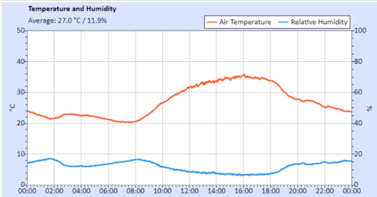
Figure 43 : Temperature and Humidity measurements.
