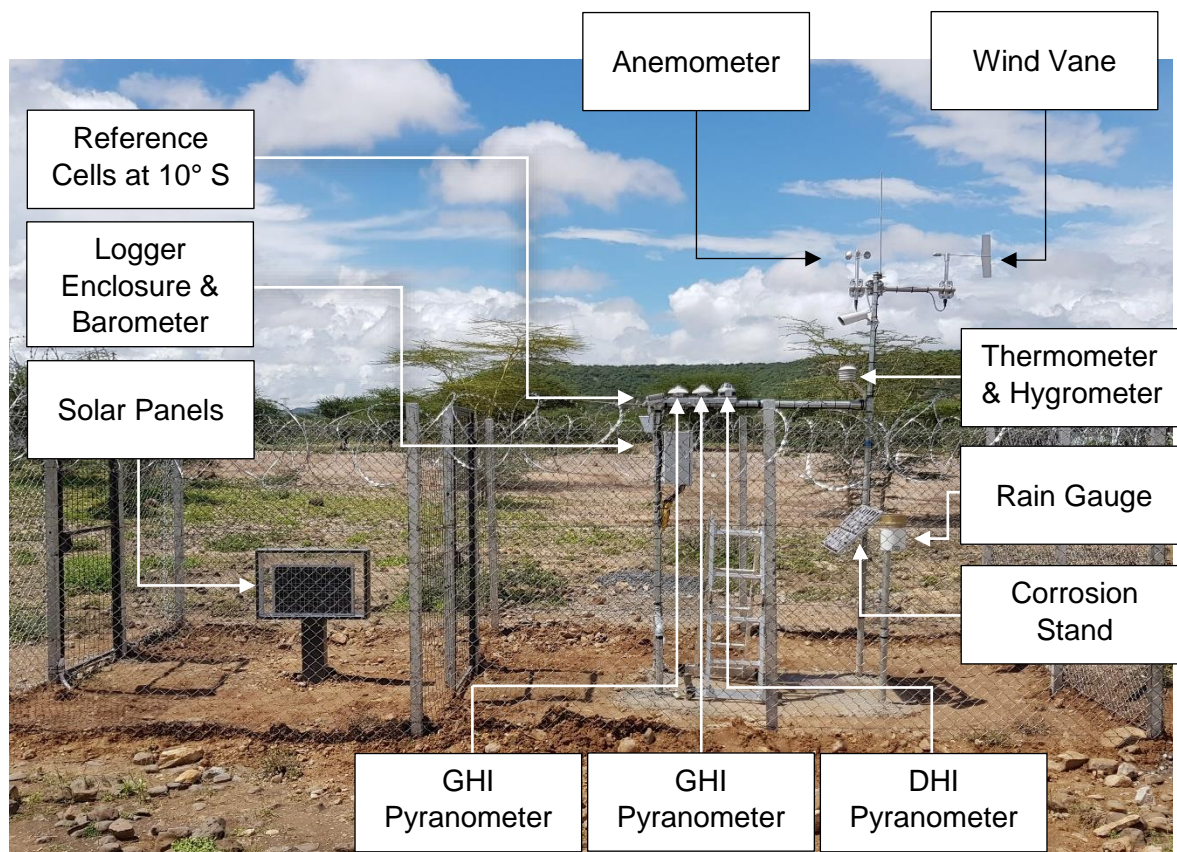
Figure 6: Station Summary
