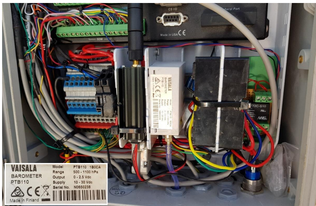
Figure 14: Barometer
