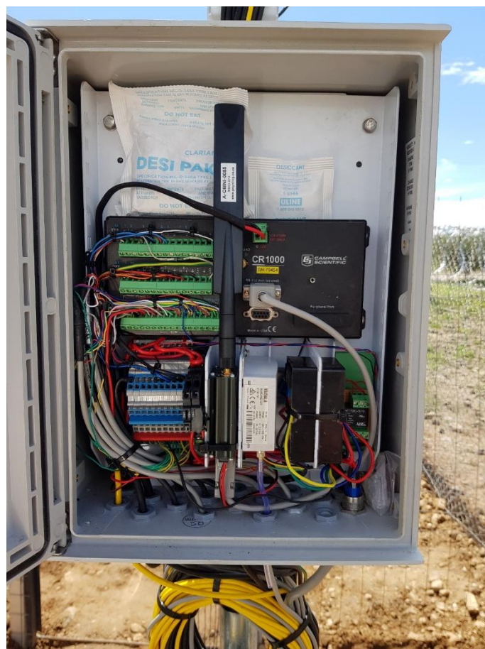
Figure 17: Logger Enclosure
