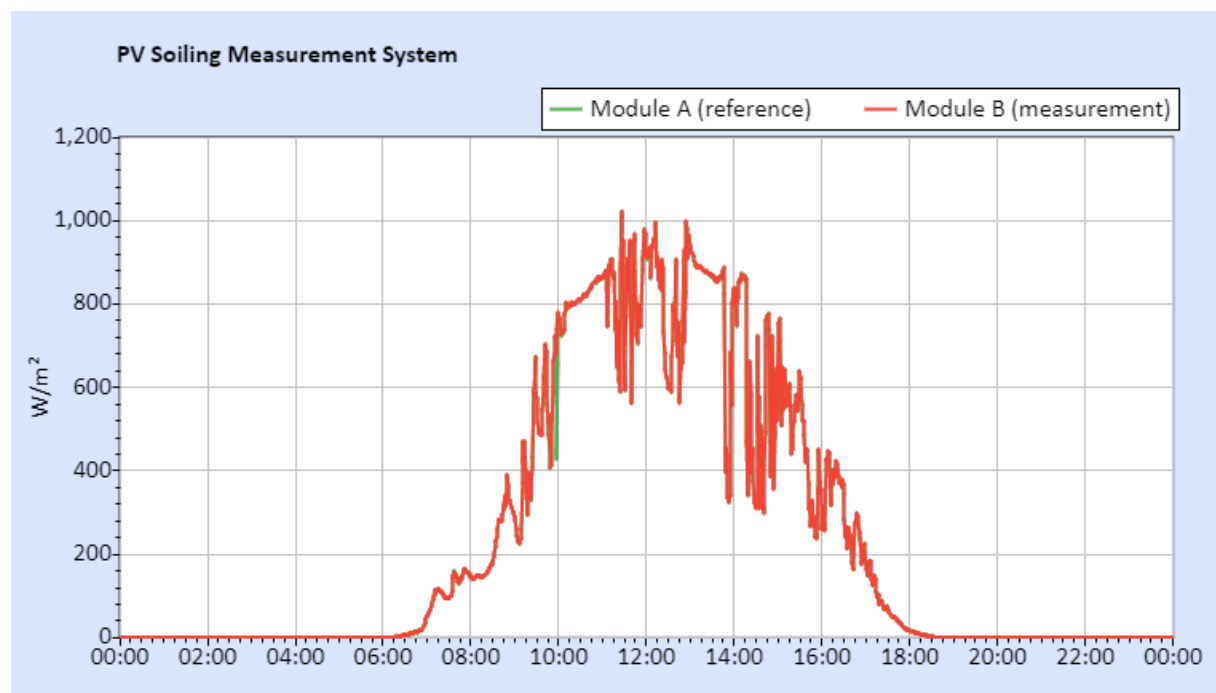
Figure 47 : PV soiling measurements.
