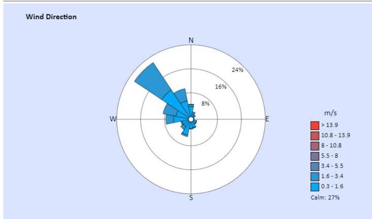
Figure 46 : Wind direction measurement.
