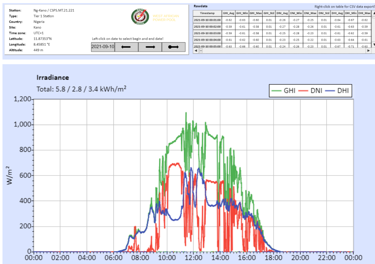
Figure 41 : Irradiance measurement. GHI, DNI and DHI.
