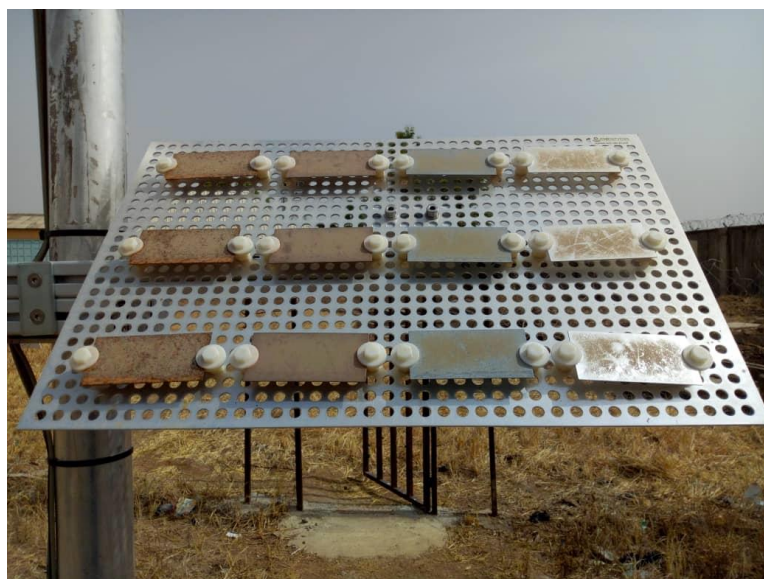
Figure 87: Echantillonneur de corrosion / Corrosion sampler.
