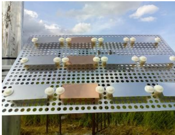
Figure 69: Echantillonneur de corrosion / Corrosion sampler.
