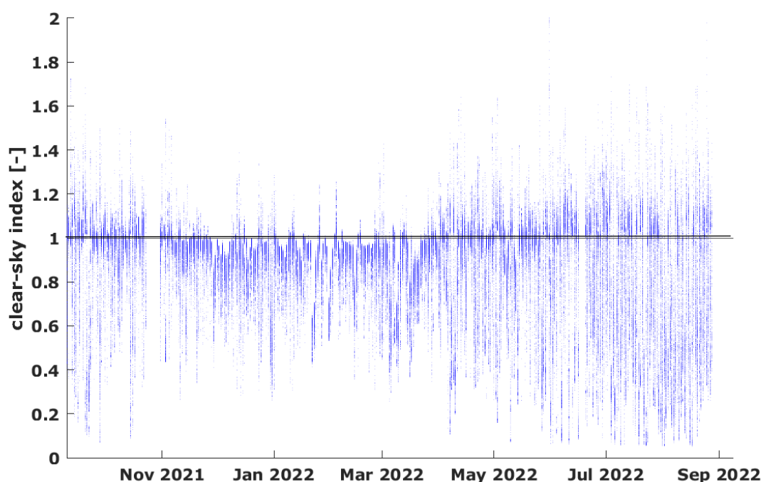
Figure 39: Indice ciel clair pour la GHI (resolution 1min) / Clear-sky index for the GHI (1min resolution).
