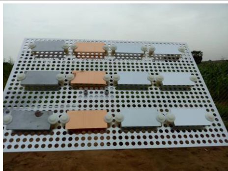
Figure 69: Echantillonneur de corrosion / Corrosion sampler.
