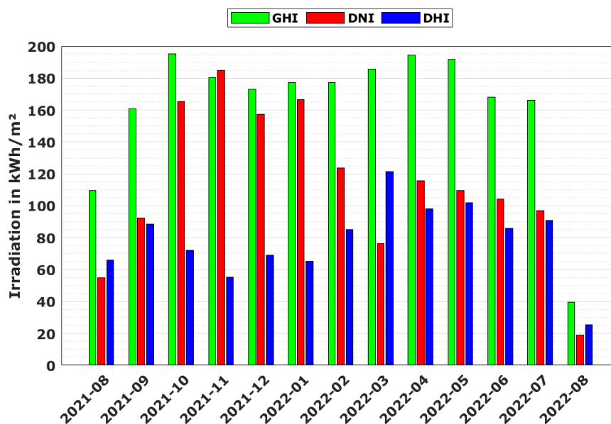
Figure 21: Totals mensuels de l'irradiation / Monthly irradiation sums.
