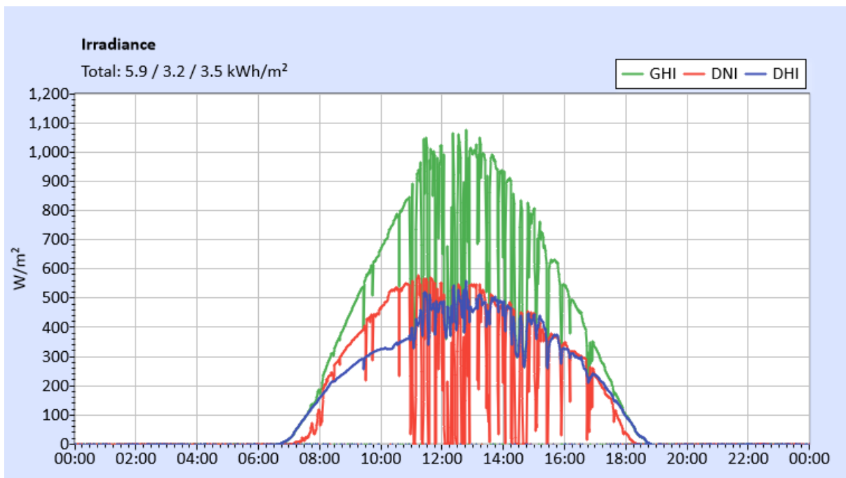
Figure 13: Mesure de l'irradiance. GHI, DNI et DHI / Irradiance measurement. GHI, DNI and DHI.
