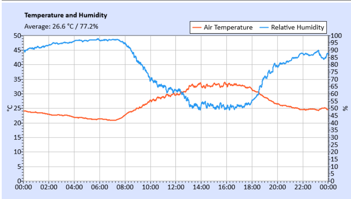
Figure 43 : Temperature and Humidity measurements.
