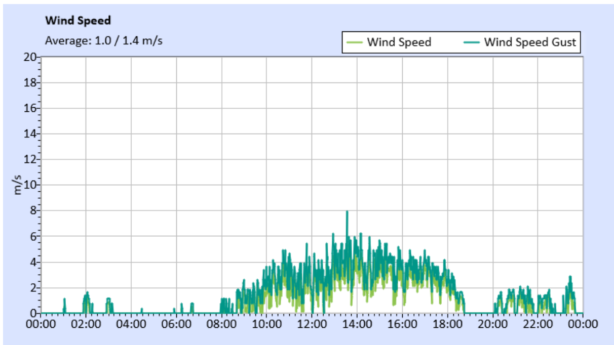
Figure 46 : Wind speed measurement.
