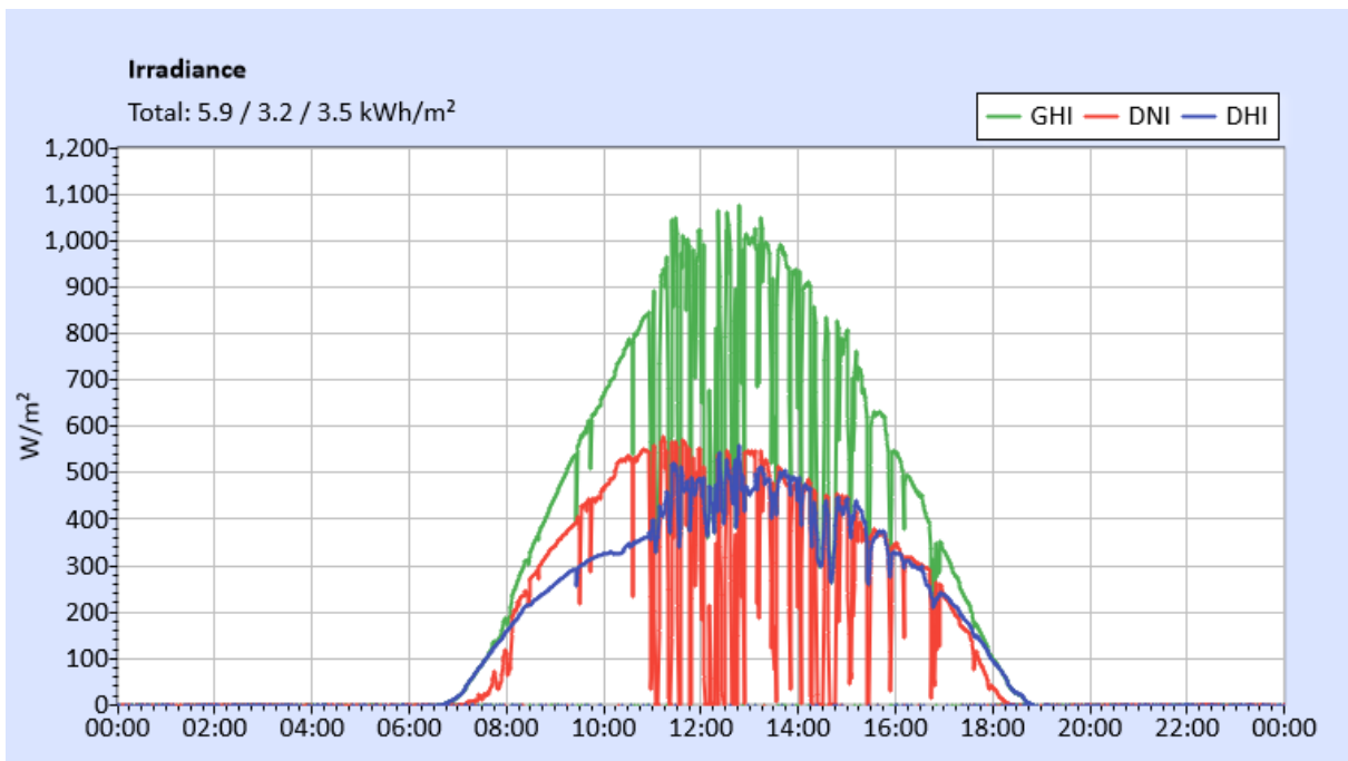
Figure 42 : Irradiance measurement. GHI, DNI and DHI.
